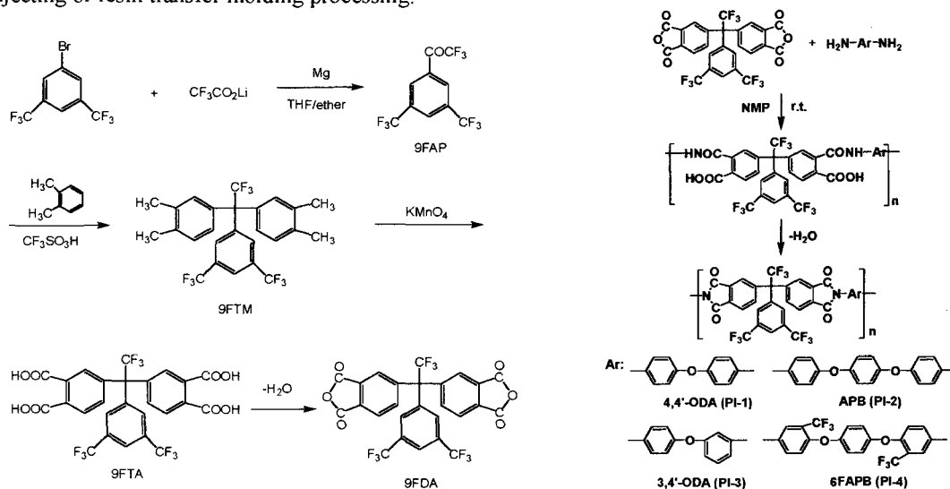
Scheme 1. Synthesis of fluorinated aromatic dianhydrides. Scheme 2. Preparation of aromatic polyimides.
