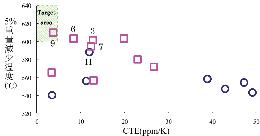
図3 T_d^5 -CTEダイアグラム: (○)従来のPI系、(□)BO基含有PI, 3: NTDA/2A4ABO, 6: NTDA/4ABO, 7: s -BPDA/DABBO, 9: NTDA/2A4ABO(50);DABBO(50)
